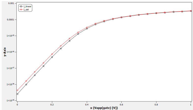
Figure 4: DIBL curve of DMG SOI MOSFET.
