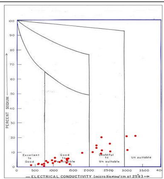
Fig. 21: Classification of Ground Water in the Study Area During Post-monsoon (After Wilcox).
