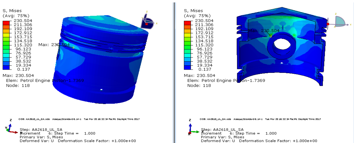
Fig. 4: The stress distribution contours for AA2618 material at 5Mpa pressure.
