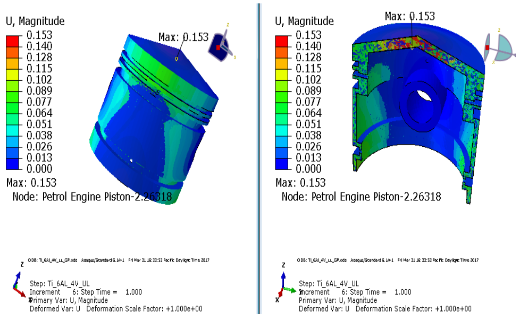
Fig. 21: The Displacement distribution contours for Ti – 6Al – 4V material at 15Mpa.
