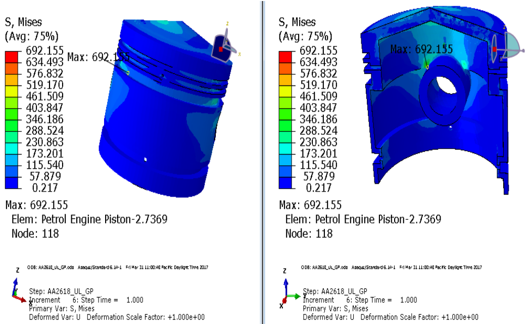
Fig. 8: The stress distribution contours for AA2618 material at 15Mpa pressure.
