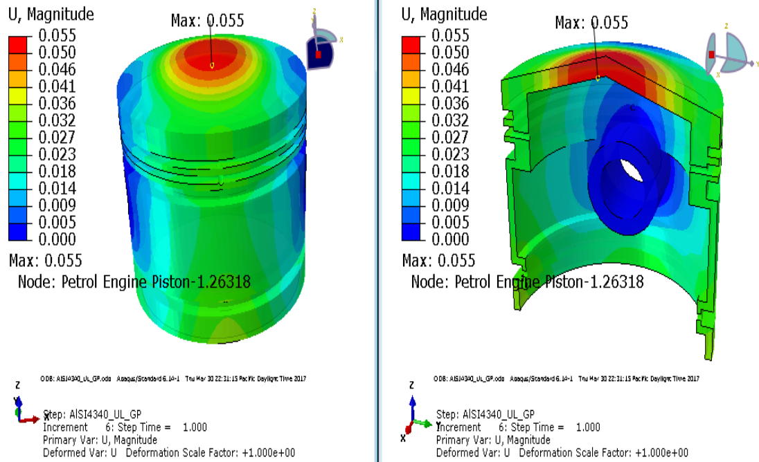
Fig. 13: The Displacement distribution contours for AISI4340 material at 10Mpa pressure.
