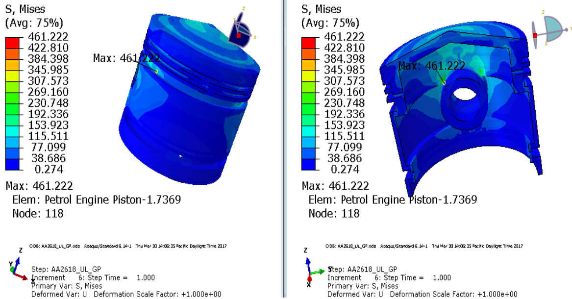
Fig 6: The stress distribution contours for AA2618 material at 10Mpa pressure.
