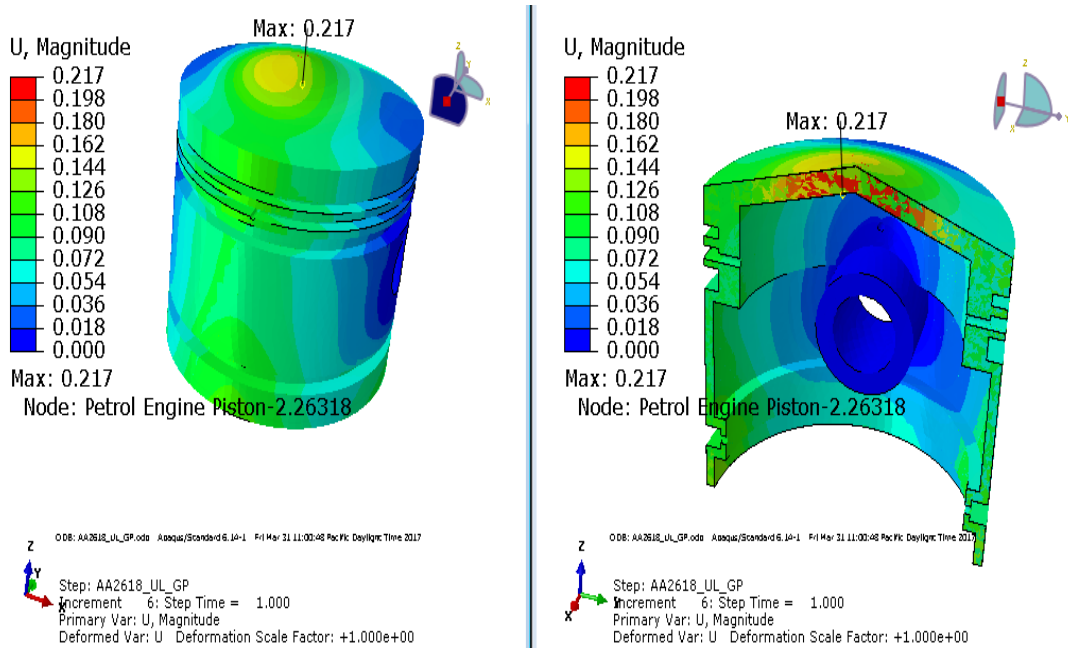
Fig. 9: The Displacement distribution contours for AA2618 material at 15Mpa pressure.
