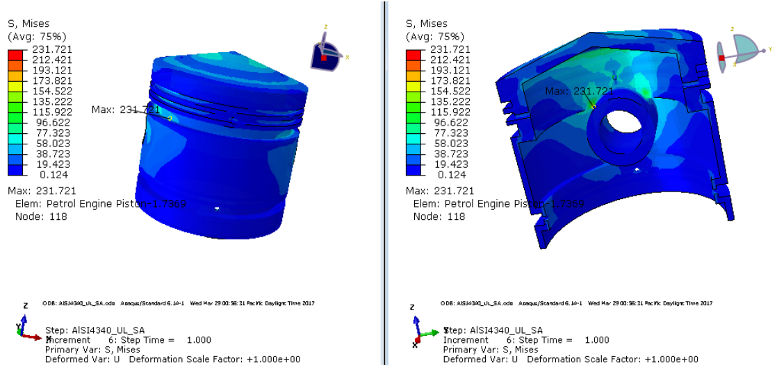
Fig. 10: The stress distribution contours for AISI4340 material at 5Mpa pressure.
