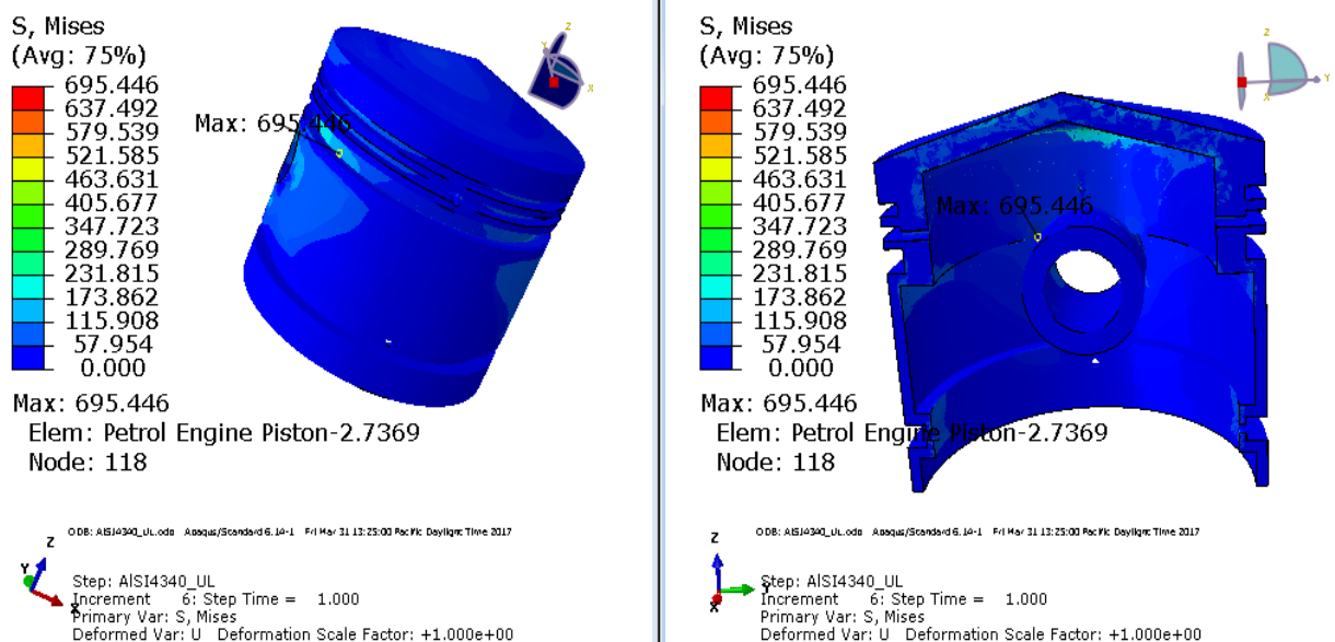
Fig. 14: The Stress distribution contours for AISI4340 material at 15 Mpa pressure.
