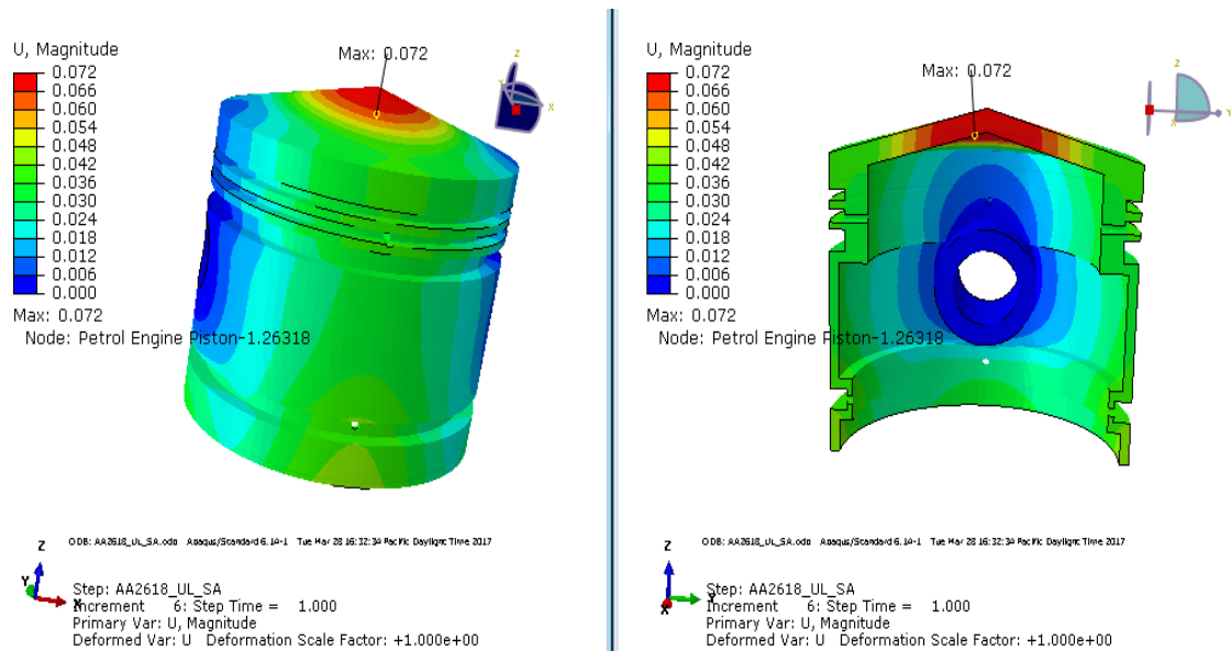
Fig. 5: The displacement distribution contours for AA2618 material at 5Mpa pressure.
