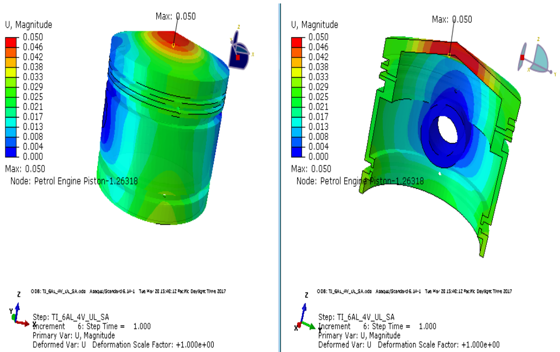
Fig. 17: The Displacement distribution contours for Ti – 6Al – 4V material at 5Mpa.
