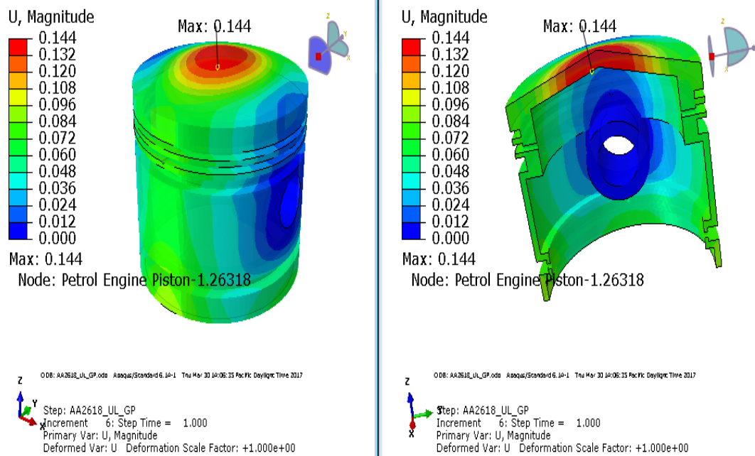
Fig 7: The Displacement distribution contours for AA2618 material at 10Mpa pressure.
