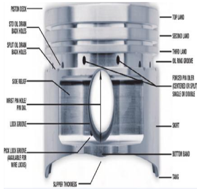
Fig. 1: Basic Components of A Piston.
