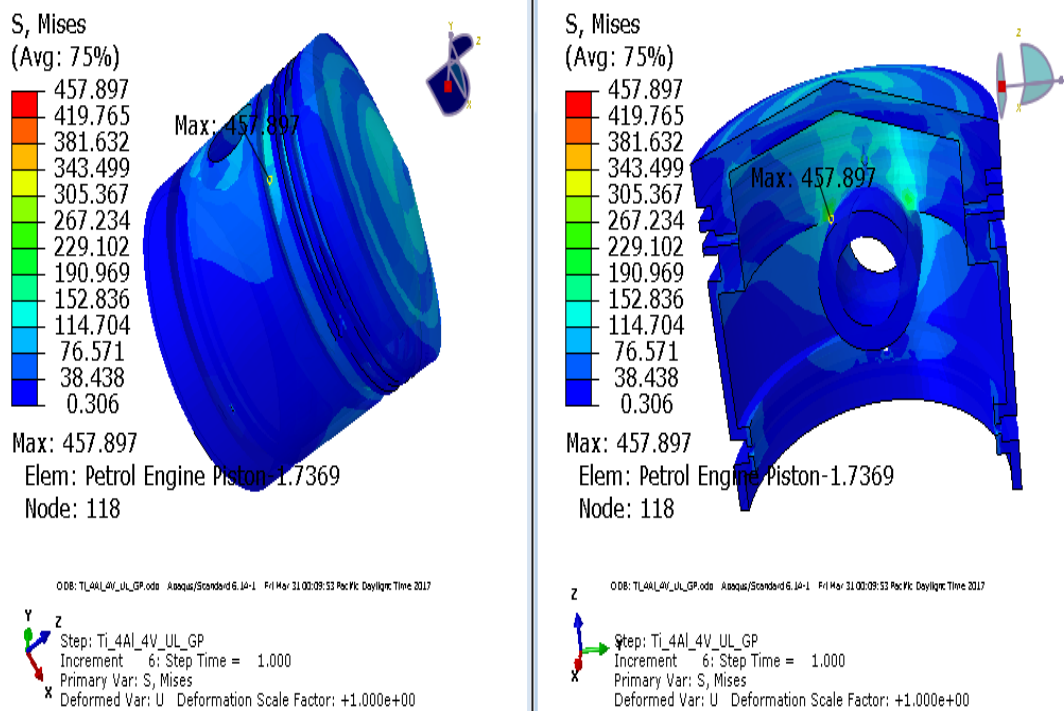
Fig. 18: The Stress distribution contours for Ti – 6Al – 4V material at 10Mpa.
