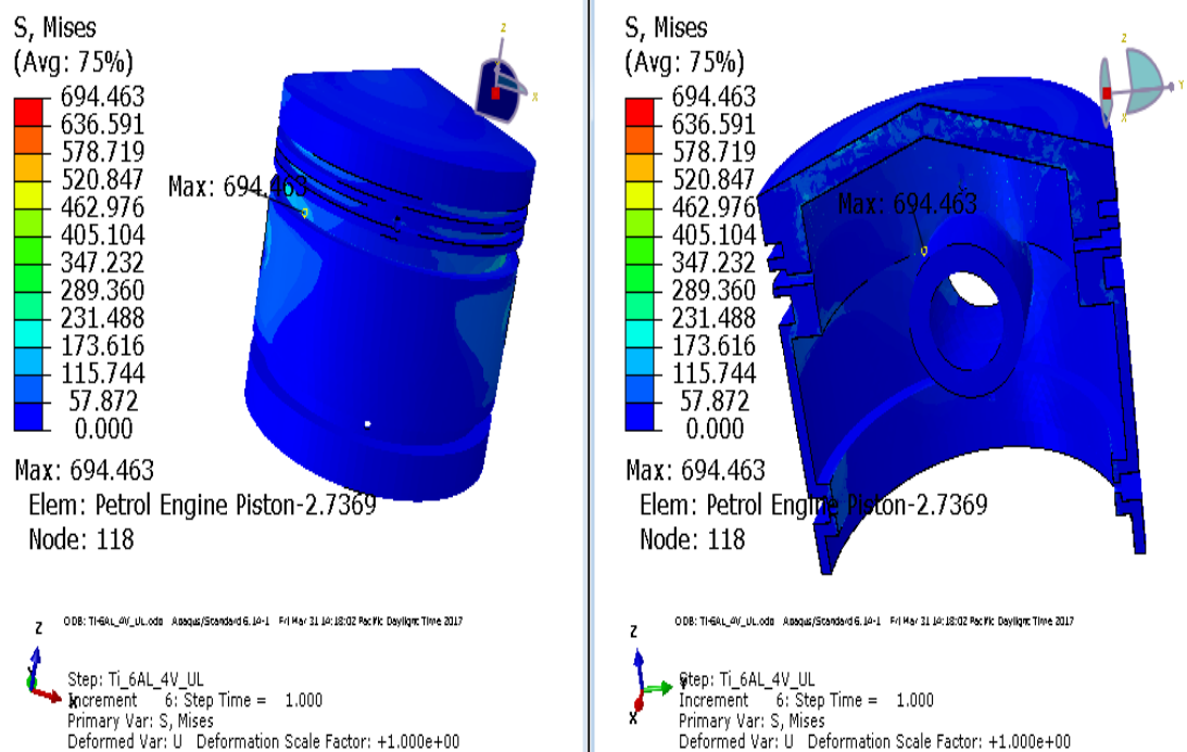
Fig. 20: The Stress distribution contours for Ti – 6Al – 4V material at 15Mpa pressure.
