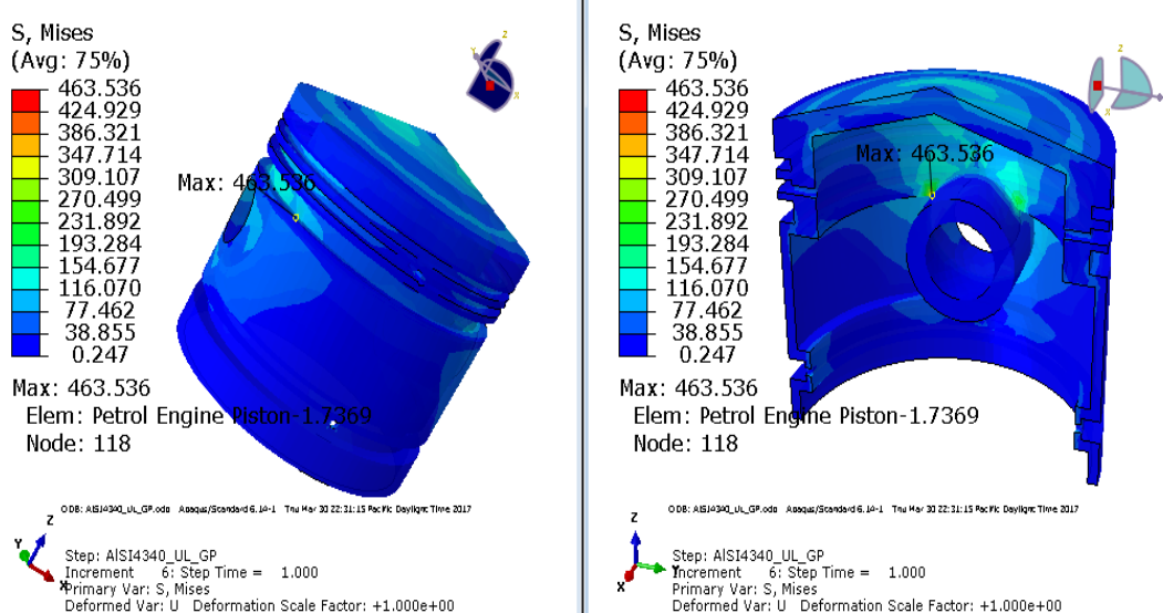
Fig. 12: The Stress distribution contours for AISI 4340 material at 10Mpa pressure.
