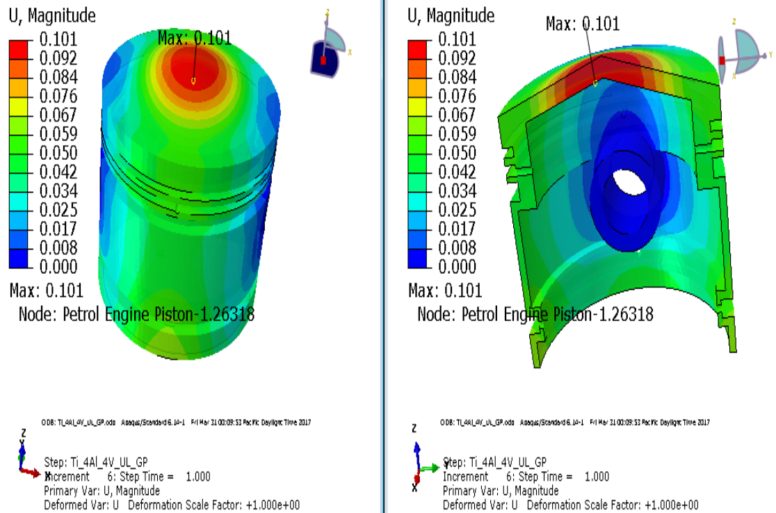
Fig. 19: The Displacement distribution contours for Ti – 6Al – 4V material at 10Mpa.
