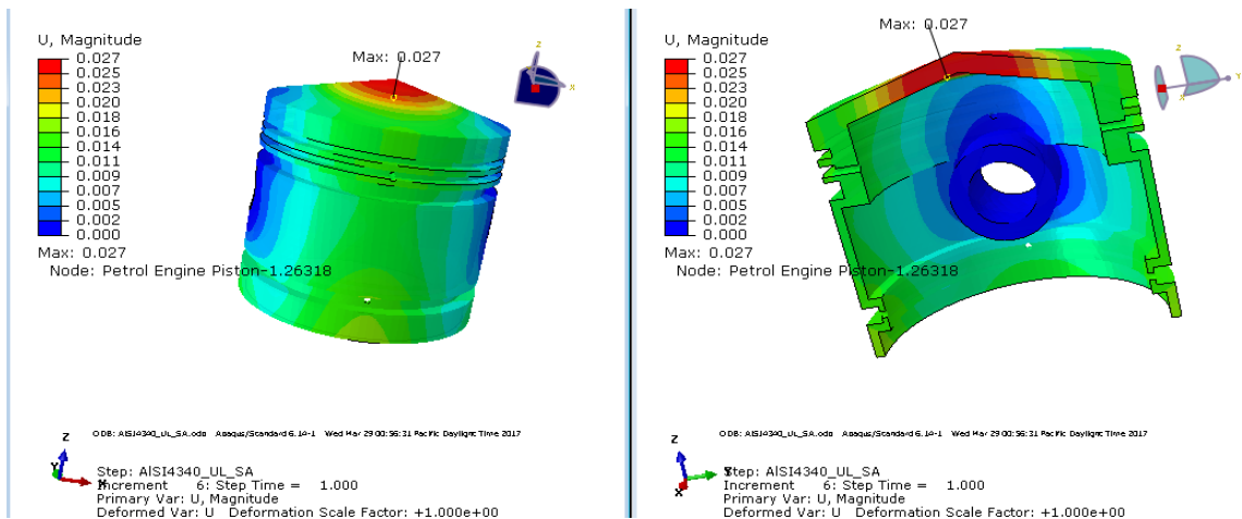
Fig. 11: The Displacement distribution contours for AISI4340 material at 5Mpa pressure.
