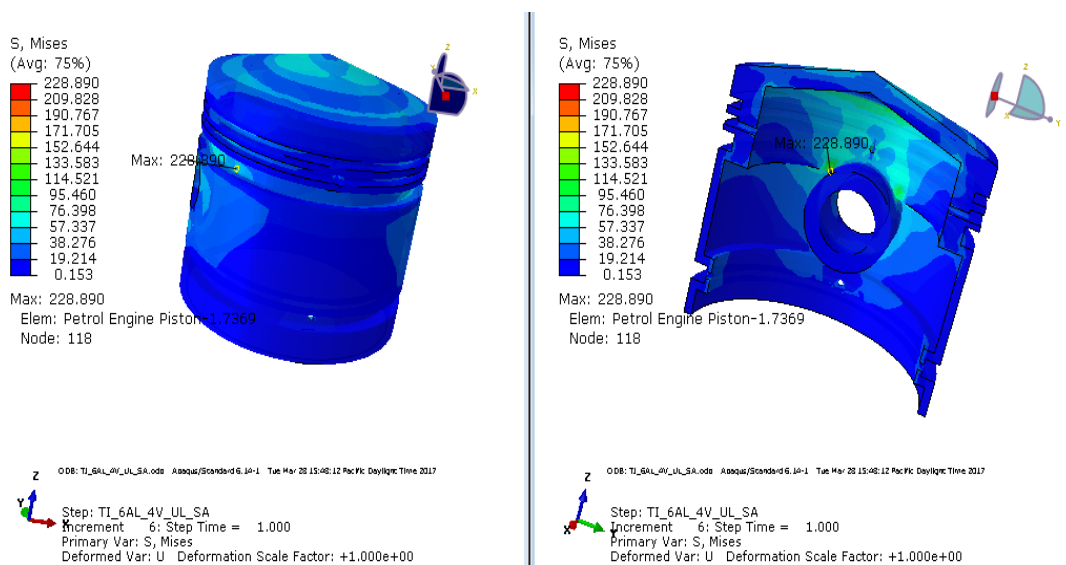
Fig. 16: The Stress distribution contours for Ti – 6Al – 4V material at 5Mpa pressure.
