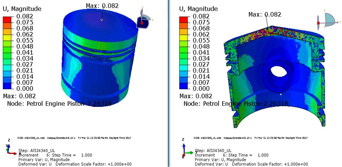
Fig. 15: Displacement distribution contours for AISI4340 material at 15 Mpa pressure
