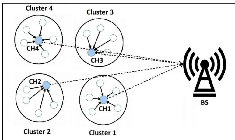
Fig. 13: LEACH Clustering. [39]
