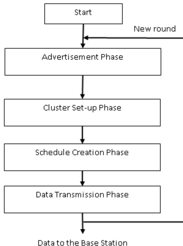
Fig. 14: LEACH Flowchart. [40]
