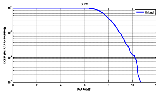
Fig. 3: PAPR of conventional OFDM system model.
