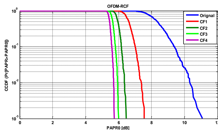
Fig. 4: PAPR of OFDM with RCF with four clipping and filtering process.
