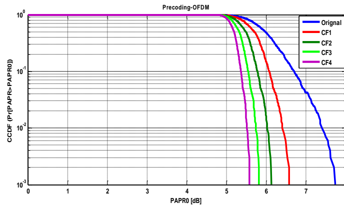
Fig. 5: PAPR of OFDM with precoding plus RCF.
