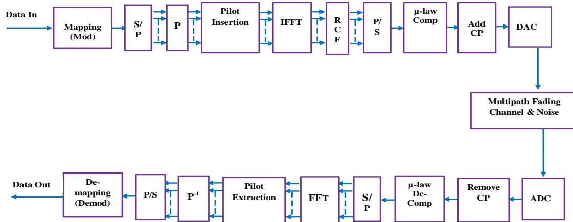
Fig. 1: Proposed OFDM system model for PAPR reduction.
