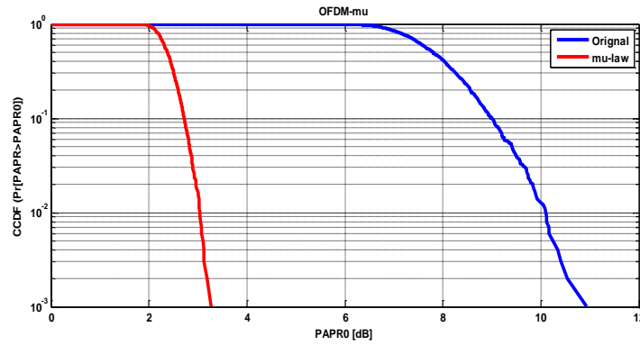
Fig. 6: PAPR in OFDM with Mu-law compandding.
