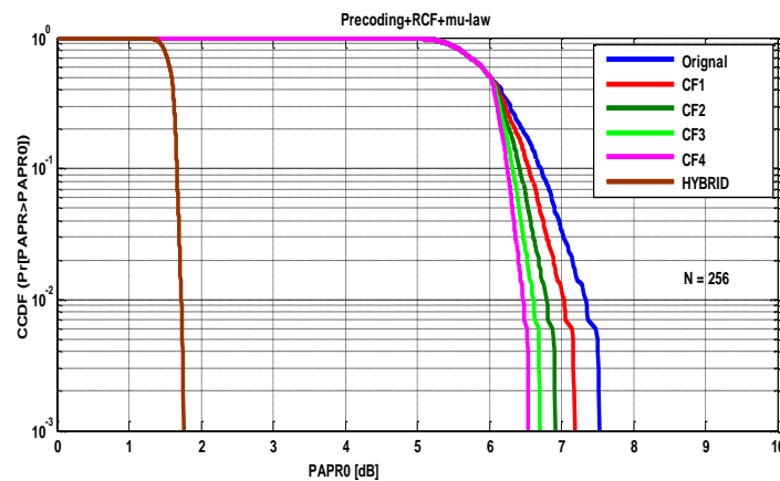
Fig. 7: PAPR OFDM with precoding plus RCF plus Mu-law.
