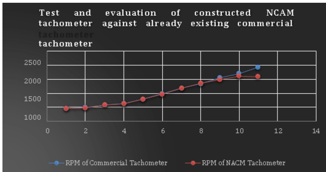
Figure 7: RPM of new tachometer vs RPM of commercial tachometer.
