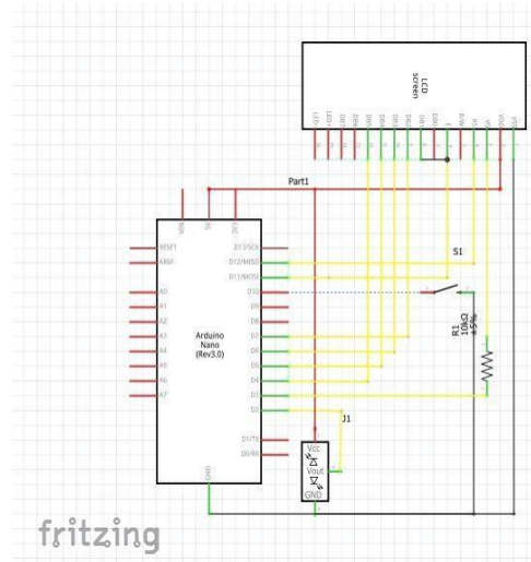
Figure 1: Fritzing diagram of the circuitry.
