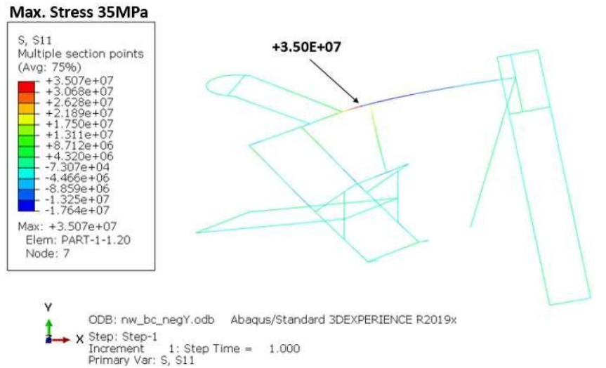
Figure 5: Maximum stress observed for 1g load.
