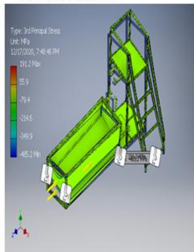
Figure 11 3rd Principal Stress
