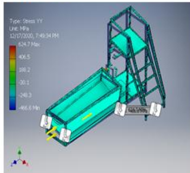
Figure 15: Stress YY
