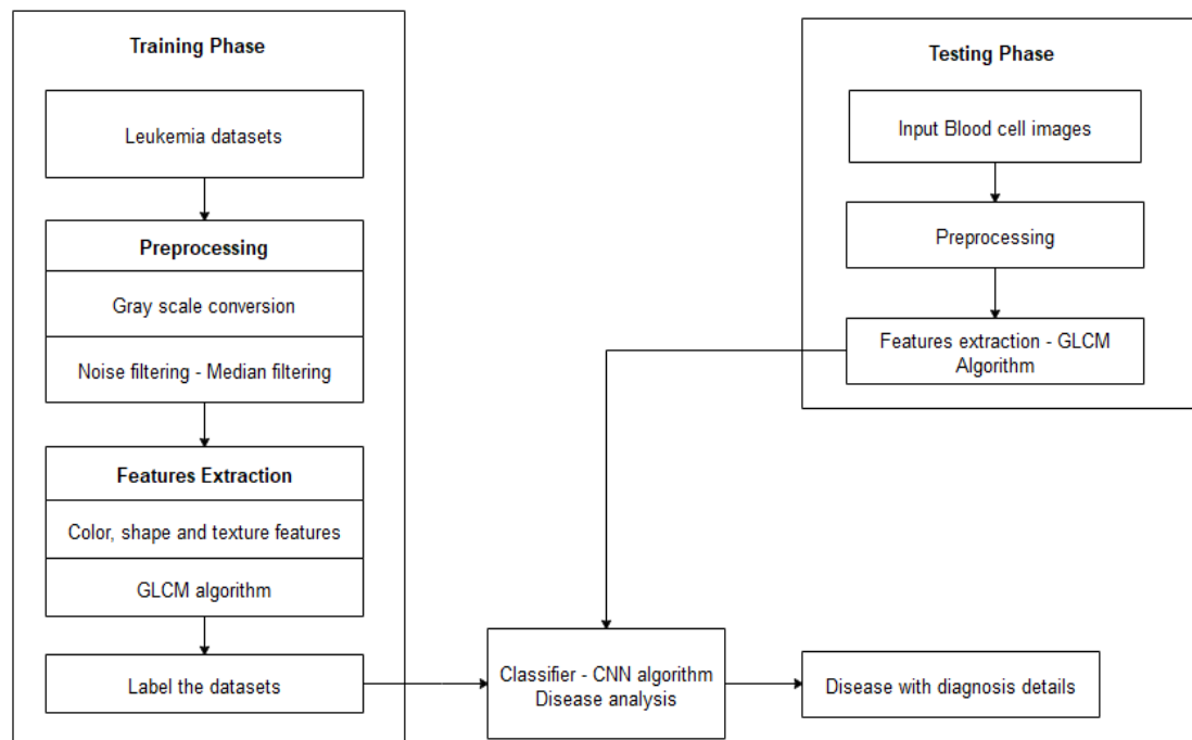
Figure 3: System architecture.
