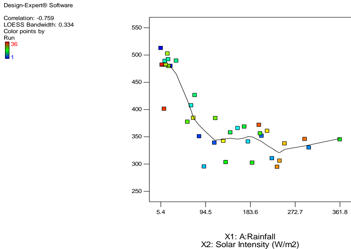
Figure 1: Correlation Analyses of Rainfall and Solar Intensity.
