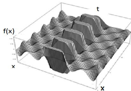
Fig. 3: During the motion, the packet f(x) will Appear and Disappear periodically.
