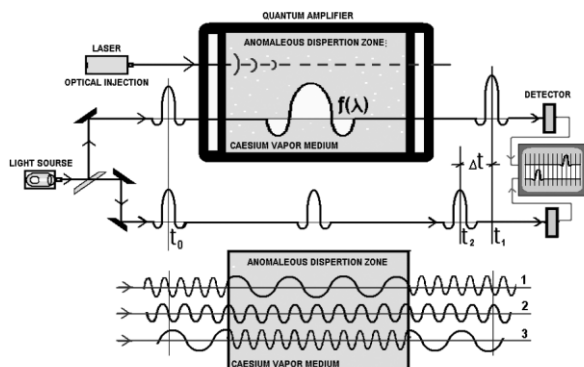
Fig. 6: Experiments of L. Wang superluminal light propagation.
