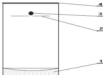
Fig. 10: Scheme of Kozyrev telescope. 1 – focusing mirror, 2 - slot, 3 - detector, 4 – light-proof lid.
