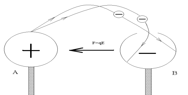
Fig. 8: Work for transferring the charge depends on the mode of Transferring and On the path.
