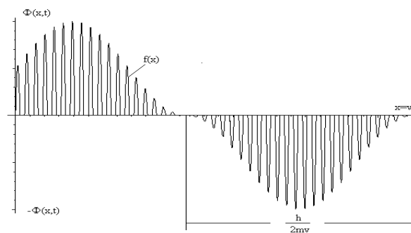
Fig. 2: Behavior of wave packet in linear dispersion medium (i.e., rather like a series of stroboscopic photographs).
