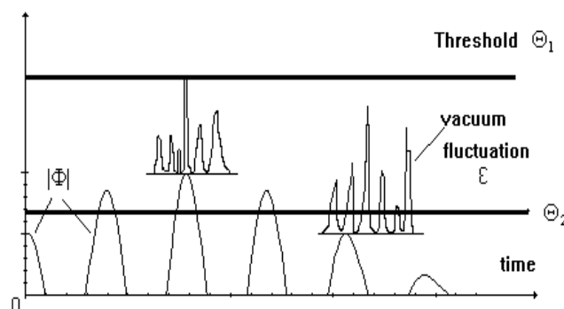
Fig. 5: Quantum measurements.
