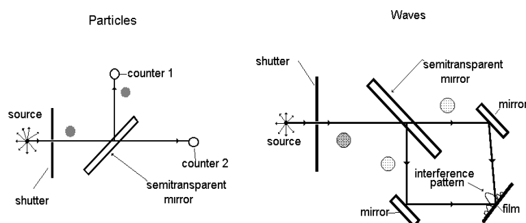
Fig. 1: Experiments with individual photons on semitransparent mirror.
