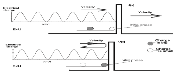
Fig. 13: Illustration of the tunnel effect.
