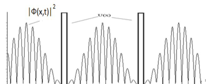
Fig. 14: Visual image of particles passing through two potential barriers - scheme of New Maxwell Demon.
