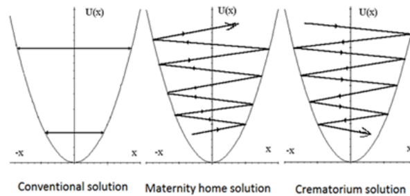
Fig. 9: Solution of UQT for harmonic oscillator.
