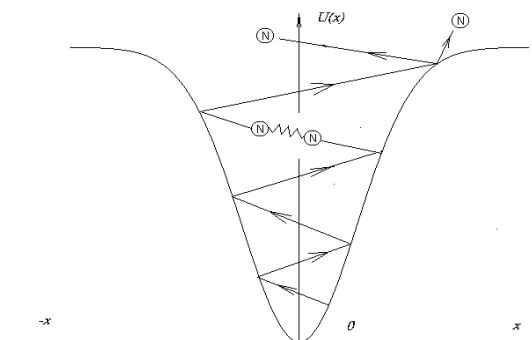
Fig. 12: Oscillation of Nitrogen molecule in potential well of catalyst.
