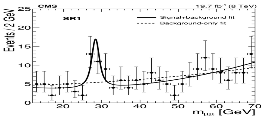
Fig. 7: Peak of energy at 28GeV.
