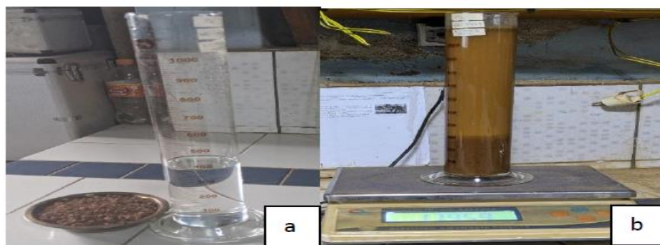
Figure 7 a) Soil Sample and Pycno cylinder b) Weighing of the Soil and Solvent content.
