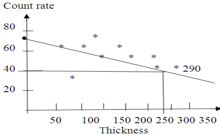
Graph -2: Strontium ( 90 Sr) Source.
