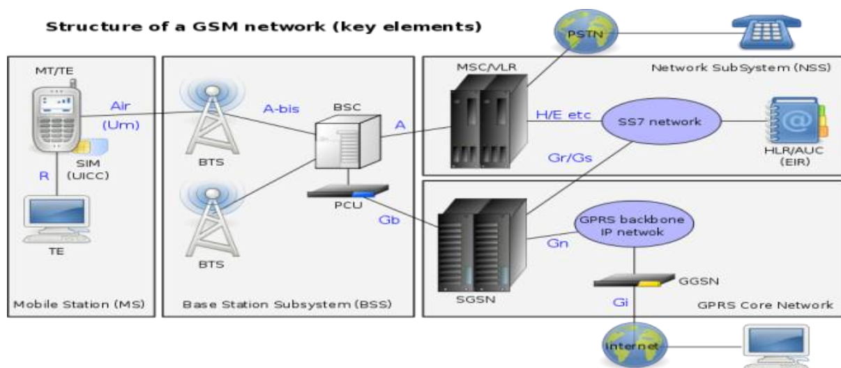
Fig: 3.1 structure of GSM network.
