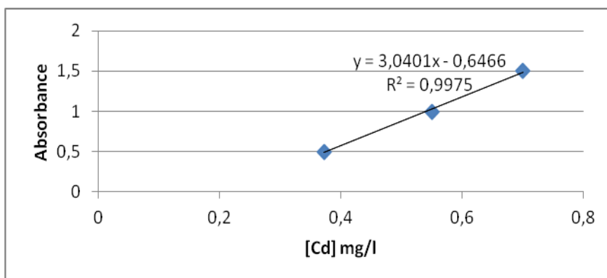
Figure N°3 : Cadmium calibration curve A = f(\text{Cd}) .
