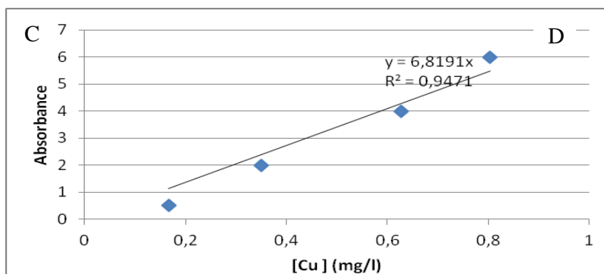
Figure N°2: Copper Calibration Copper A = f(\text{Cu}) .
