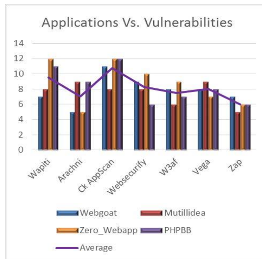
Figure 5: Web Scanning Applications Vs. Vulnerabilities.
