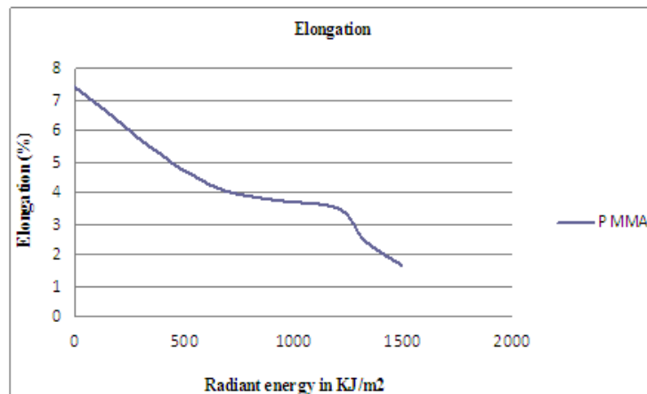
Figure 10: Overall trend of Elongation property of PMMA after exposure to weathering.
