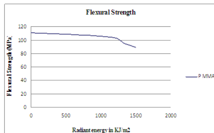
Figure 9: Overall trend of Flexural property of PMMA after exposure to weathering.
