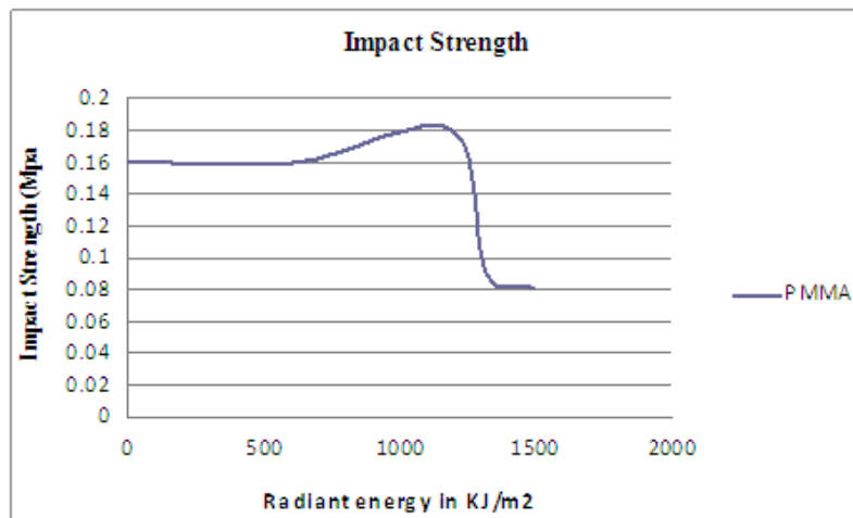
Figure 8: Overall trend of Impact property of PMMA after exposure to weathering.
