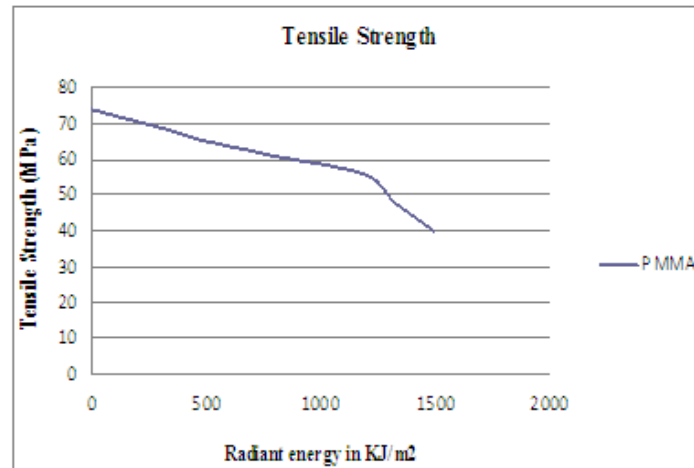
Figure 7: Overall trend of tensile property of PMMA after exposure to weathering.
