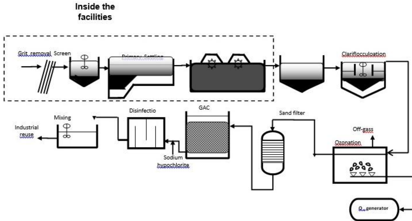
Figure 4: Sketch of IWWTP for Scenario (2).
