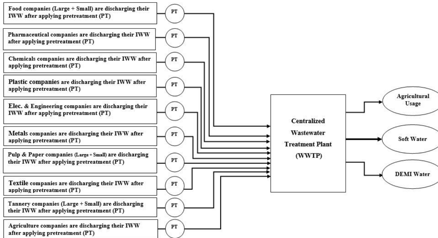
Figure 3: Scheme for Scenario (2).
