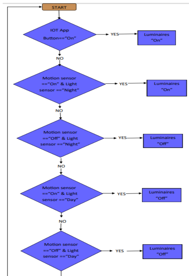
Figure 8: Flowchart.
