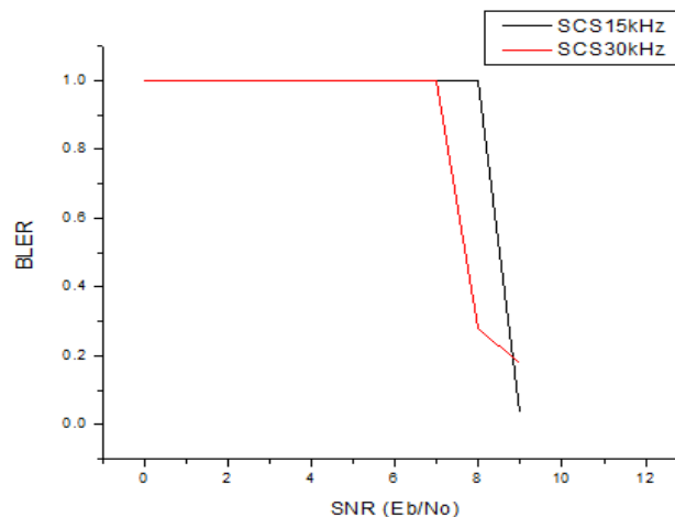
Fig. 10: BLER of 5G NR at SCS= 15 kHz and 30 kHz, MCS=16, Modulation =16 QAM and FFT size 2048.
