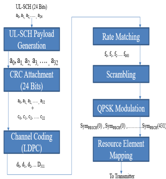
Fig. 5: PBCH Generation and Mapping.
