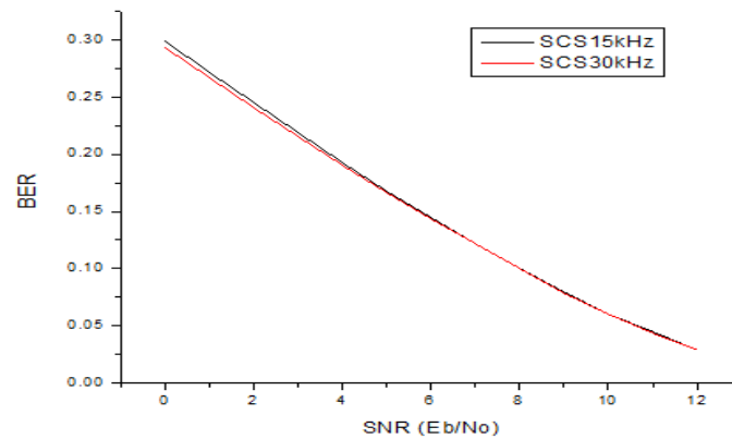
Fig. 9: BER of 5G NR at SCS= 15 kHz and 30 kHz, MCS=16, Modulation =16 QAM and FFT size 2048.
