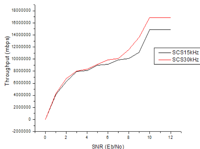
Fig. 8: Throughput of 5G NR at 15 kHz SCS, MCS=16, Modulation= 16 QAM and FFT size 2048.
