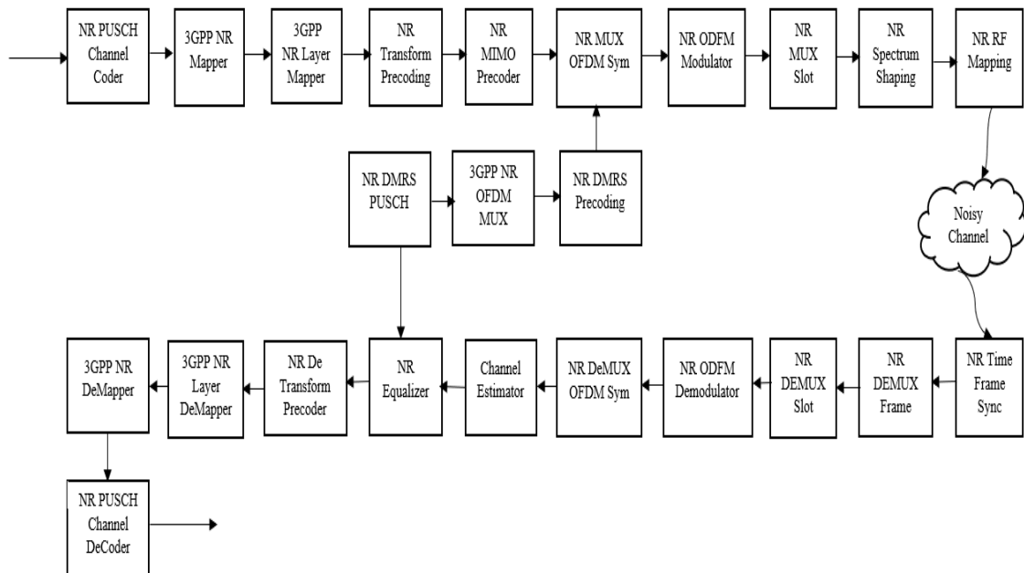
Fig. 4: Transmitter and Receiver Block Chain of 5G NR Uplink System.
