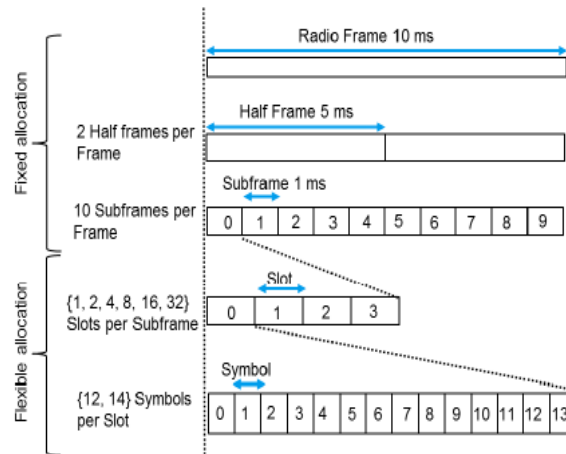
Fig. 3: Frame Structure of 5G NR Technology.
