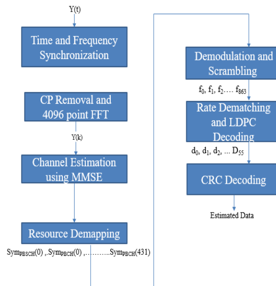
Fig. 6: Receiver Process flow of 5G NR Uplink System.
