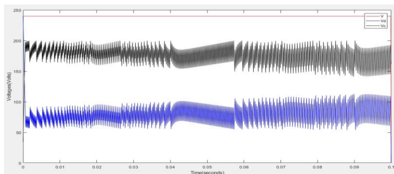
Figure 4-8: Partial discharge data for gas pressure model for a void resistance of 1e12Ω and material conductivity of 1e6Ω.
