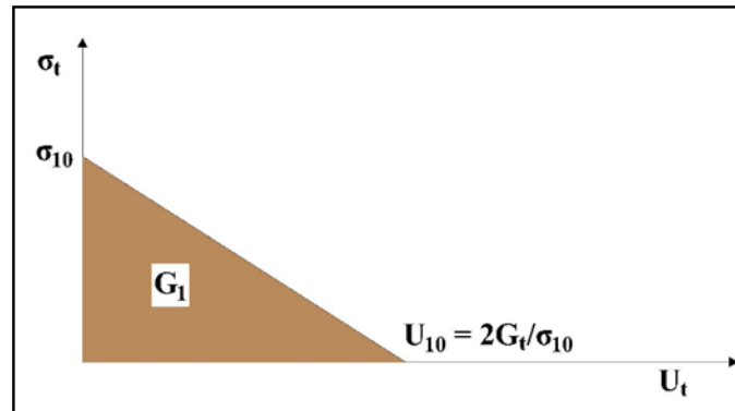
Figure 7: Post-Failure Stress-Fracture Energy Curve. [22]
