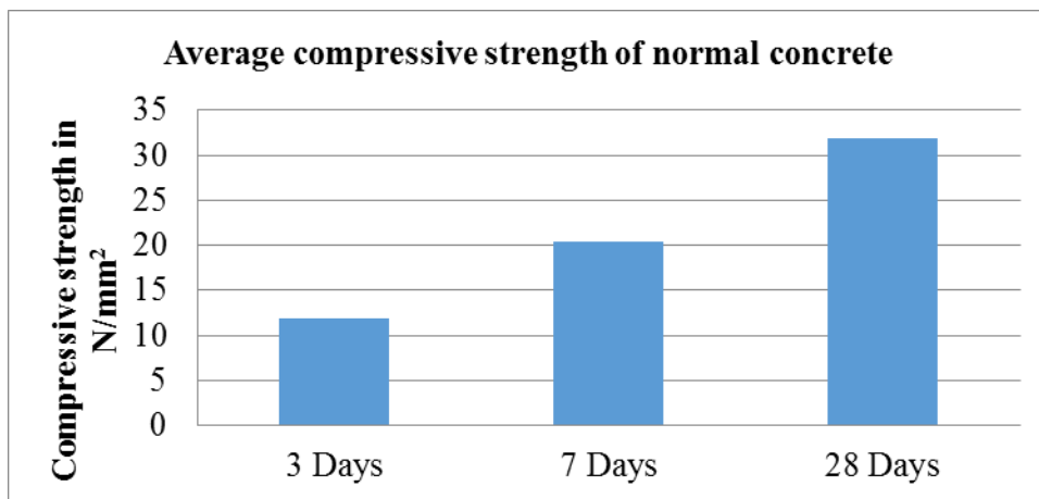
Figure 10: Compressive strength graph for conventional cement concrete.
