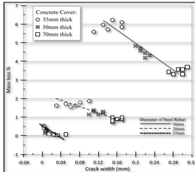
Figure 9: Effect of Crack Width on Percent Mass Loss.
