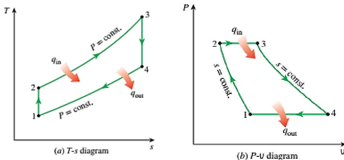
Figure 2: T-s and P-v diagrams for the ideal Brayton cycle. [2]
