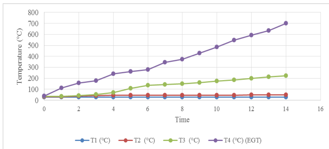
Figure 5: Temperature measurement at various times.
