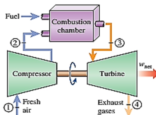
Figure 1: An open-cycle gas-turbine motor.
