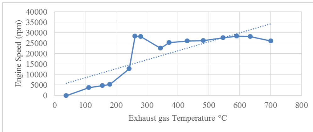
Figure 6: Motorspeed versus exhaust gas temperature data measurement.
