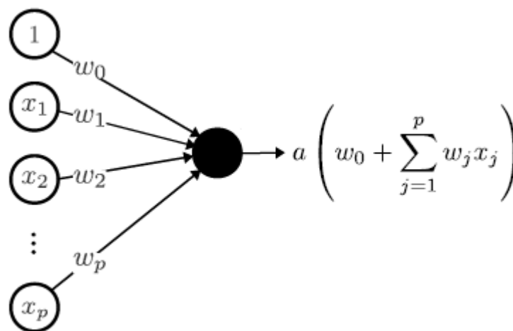
Fig. 1: Perceptron's architecture.
