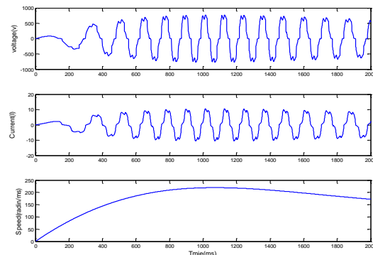
Fig.5 wind turbine modeling output
