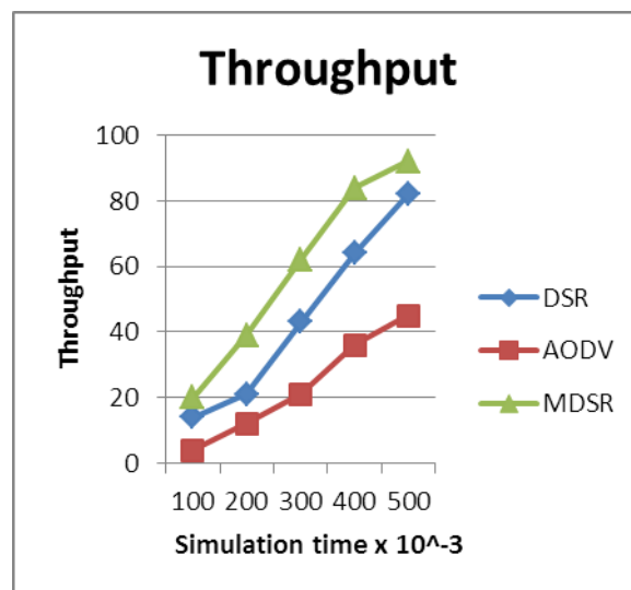
Fig. 8: Comparison of throughput between DSR, AODV and MDSR.
