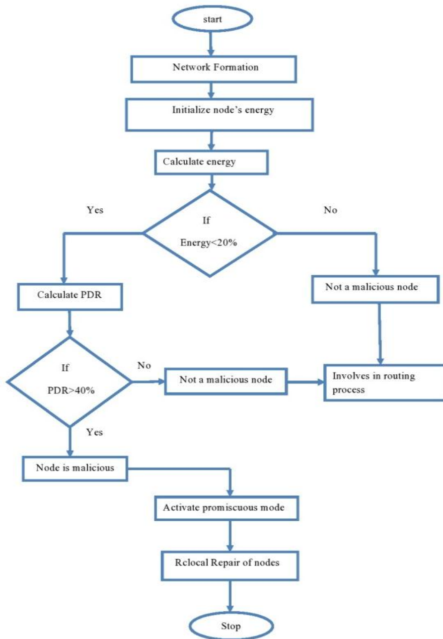
Fig. 6: Flow chart for promiscuous mode.
