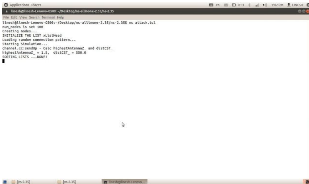
Fig. 4: Creating 100 nodes.
