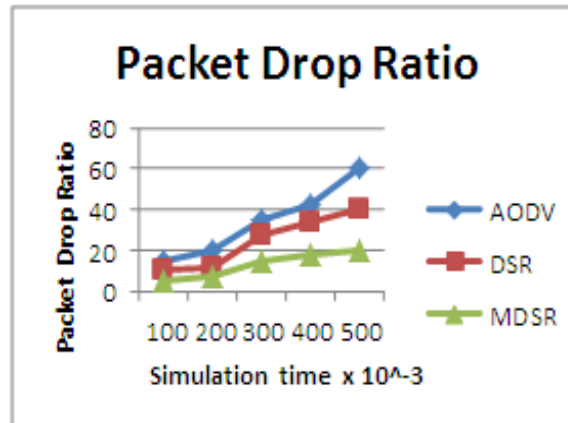
Fig. 7: Comparison of Packet Drop Ratio between DSR, AODV and MDSR.
