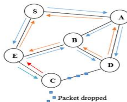
Fig 3: Packet drop by malicious node.
