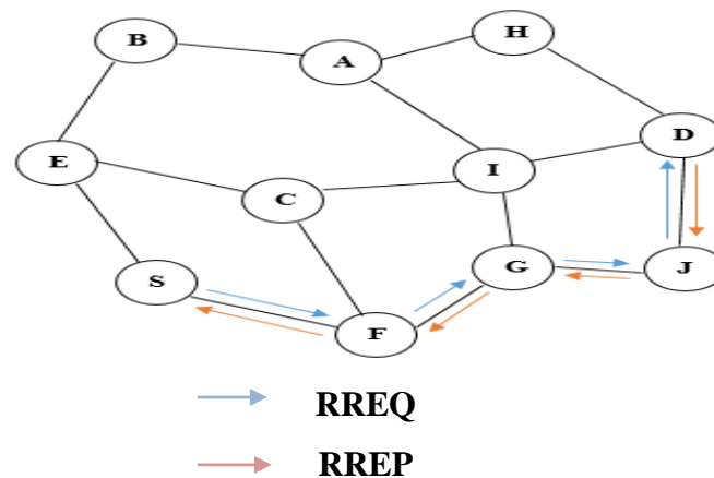
Fig. 2: Determines shortest path using Dynamic Source Routing.
