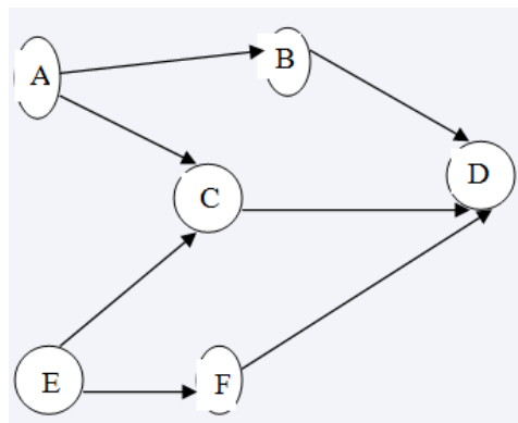
Figure 1: Disjoint Paths.
