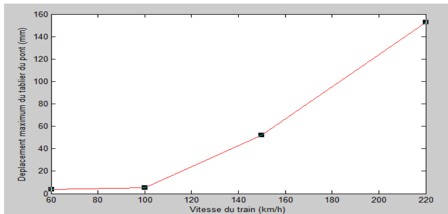
Figure 12: Simulation of maximum bridge displacements as a function of speed.
