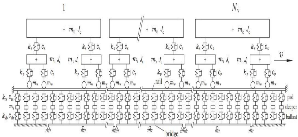
Figure 6: A typical train-track-bridge interaction system [Zeng Z.-P., 2016].
