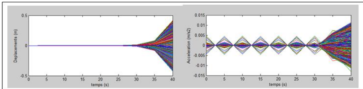
Figure 10: Time diagram of rail node displacements and accelerations at 60km/h
