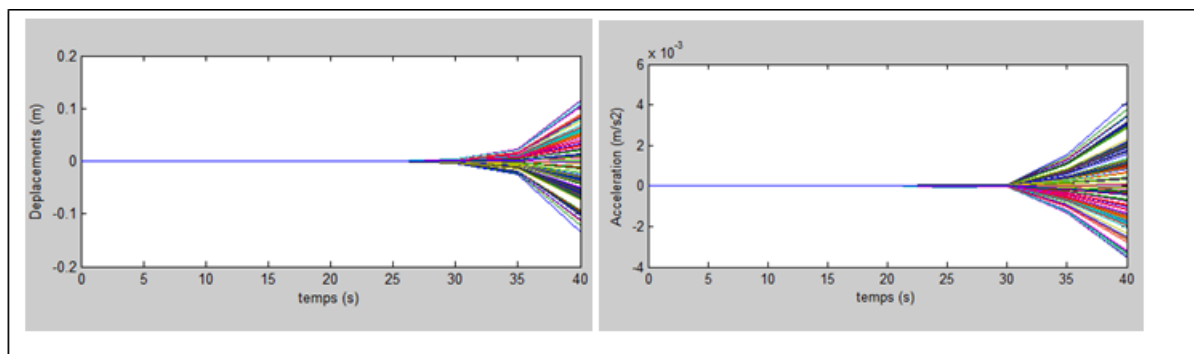
Figure 11: Time diagrams of displacements and accelerations of bridge nodes at 60km/h
