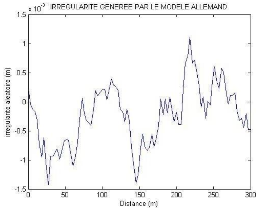
Figure 7: Track irregularities transformed by the German spectrum.
