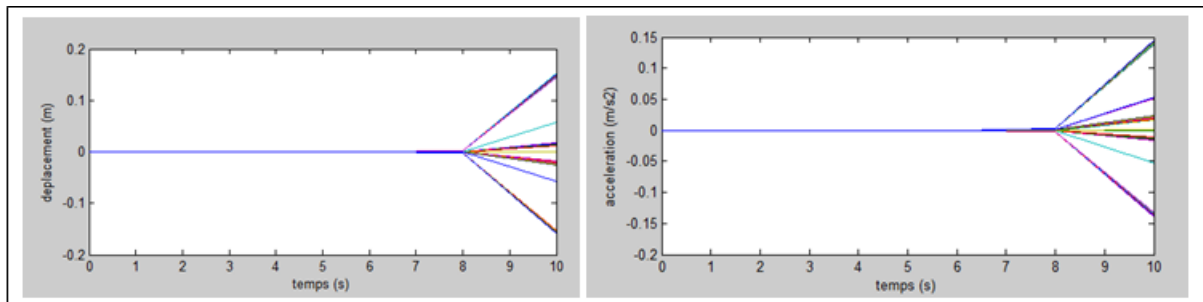
Figure 9: Time diagram of bridge node displacements and accelerations at 220km/h
