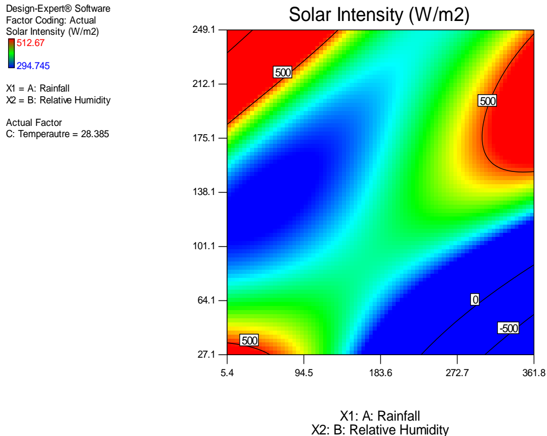
Figure 4: The Contour Plot for Rainfall and Relative Humidity.
