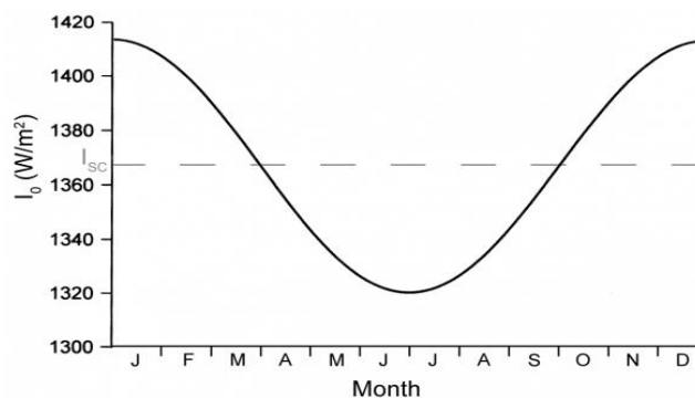
Figure 1: The variation in I_0 over the course of a year.
