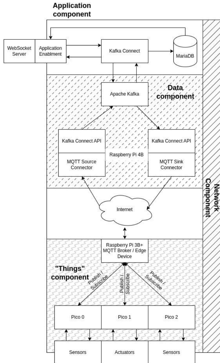
Figure 2: IoT architecture.
