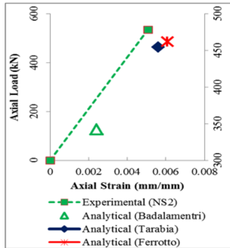
Figure 14 Comparisons between experimental results and Analytical Models for Preloaded strengthened RC column.
