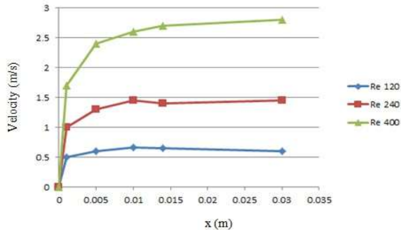
Fig. 4 velocity along the length of the channel for different values of Reynolds number.
