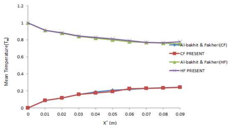
Fig. 3 comparison of mean temperatures for cold and hot fluid along length of present model and data of Al-bakhit and Fakheri. [12]
