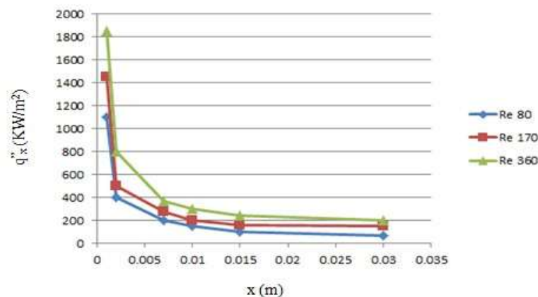
Fig. 7 variation of axial heat conduction for different values of Reynolds along the flow direction.
