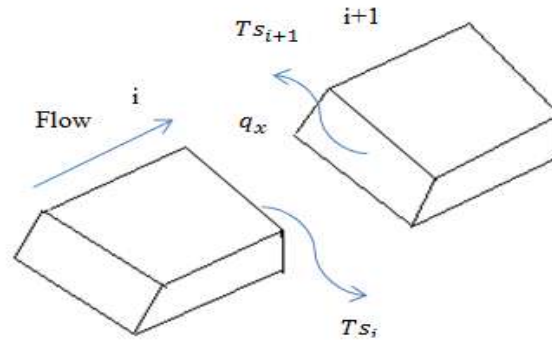
Fig. 2 Schematic of separating wall.
