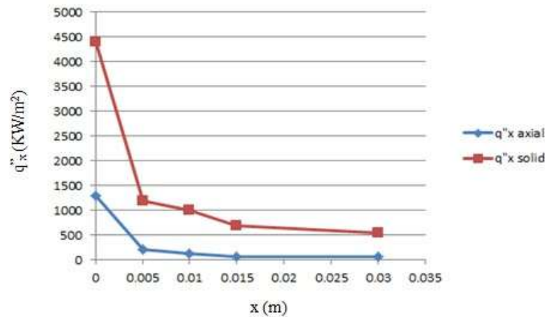
Fig. 6 axial heat conducted and heat conduction between fluids along the length of a channel.
