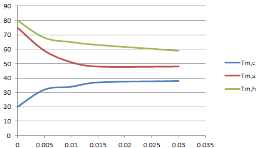
Fig.5 Temperatures of cold fluid, separating wall, hot fluid along the length of the channel.
