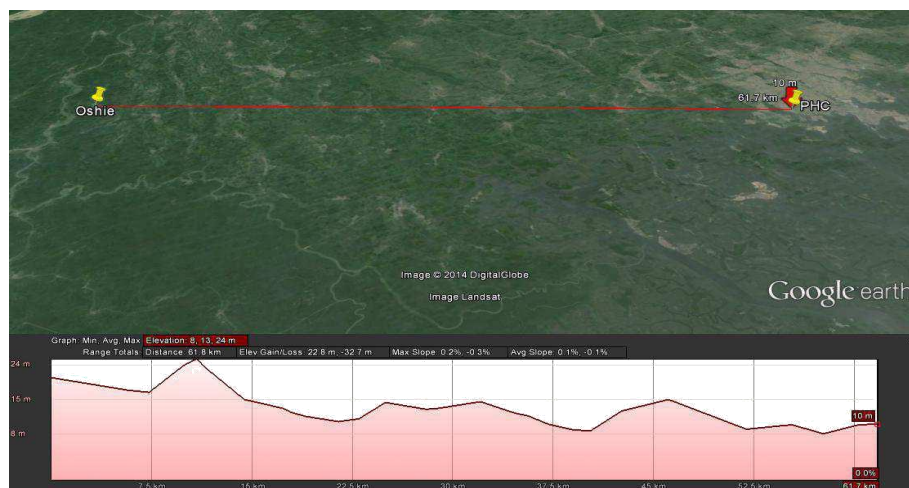
Figure 7: Oshie-Port Harcourt Microwave Link Topography and Elevation Profile (Pathloss IV, 2014).
