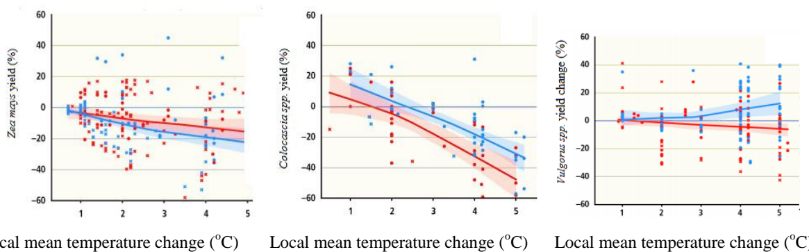
Figure 4: Percentage simulated yield change as a function of local temperature change for the three major crops for the region.
