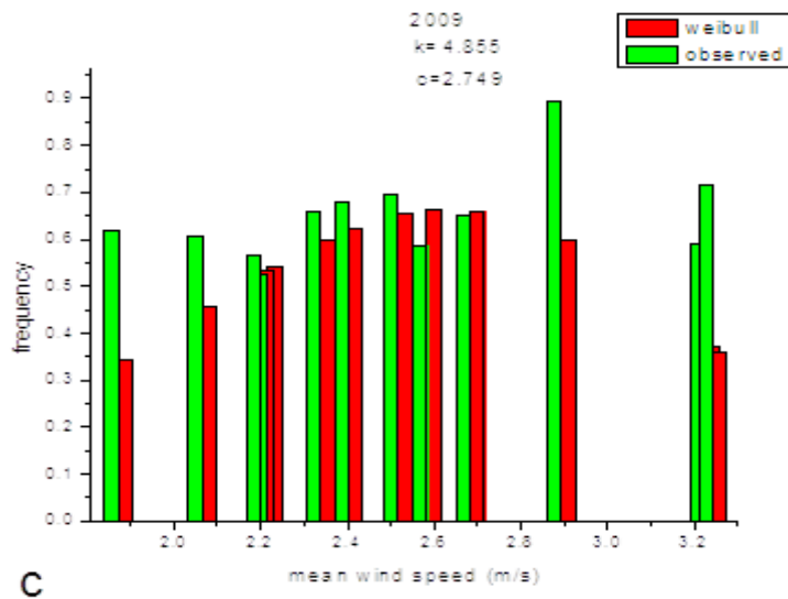
Figure 4.5: Observed and calculated wind speed frequencies for Kisumu
