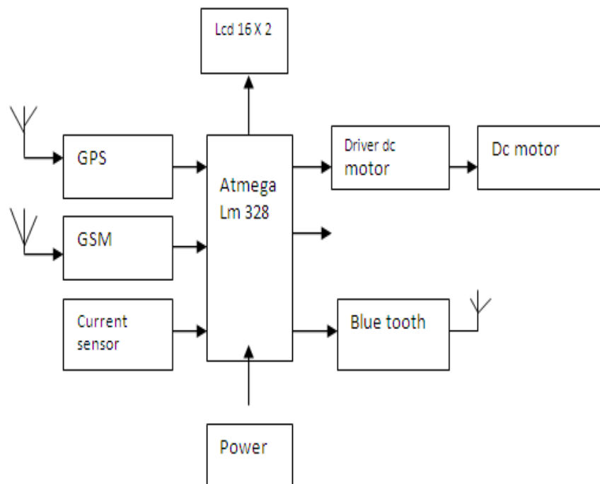
FIG (1): Block diagram of underground cable fault detection. [1]
