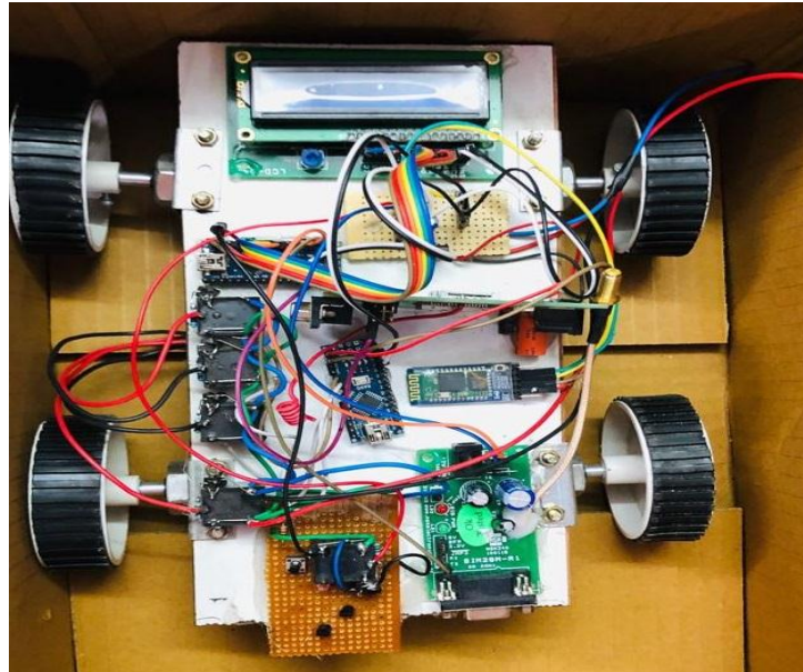
Fig. 2: Prototype of the robot.
