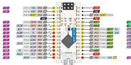
Fig. 5: Pin Diagram of Atmega328. [5]
