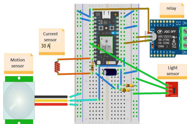
Figure 7: Connections.
