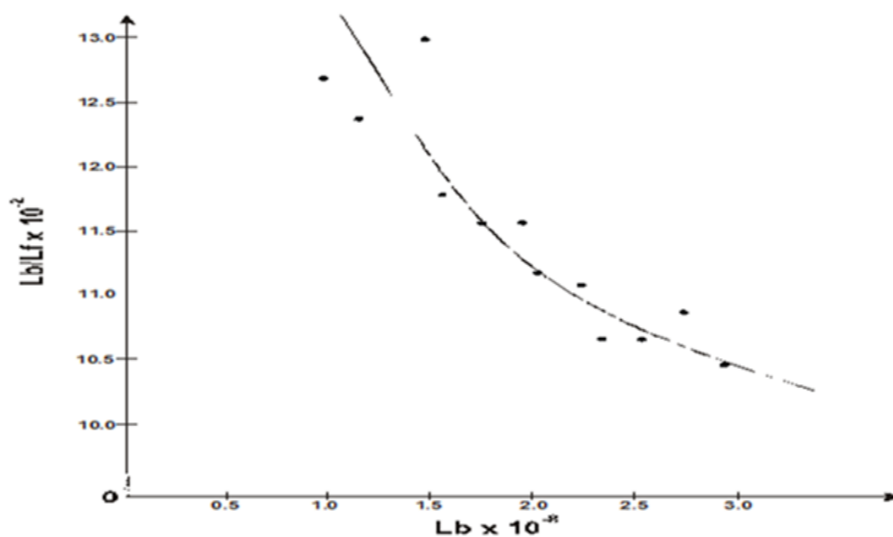
Figure 4: A scatchard plot for the binding of Dicoumarol to Bovine Serum Albumin.
