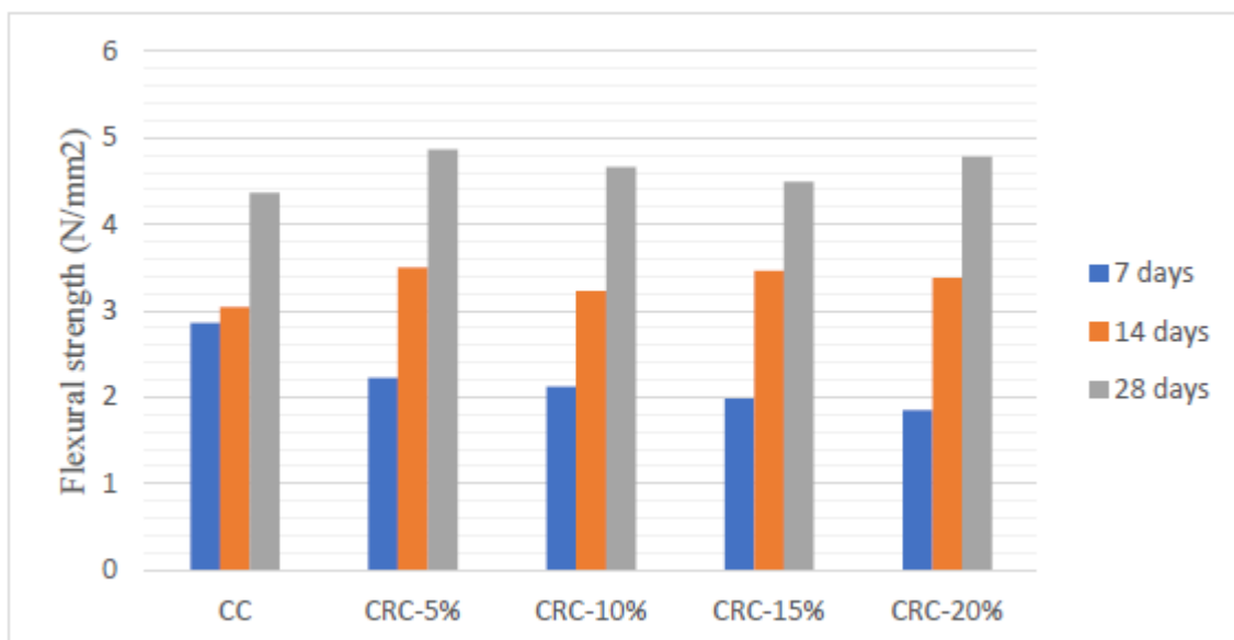
Figure 2: Flexural strength at various replacements.
