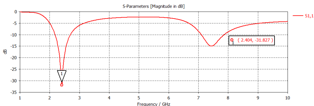
Figure 3: Return Loss Curve for the designed Half-Wave Dipole Antenna.
