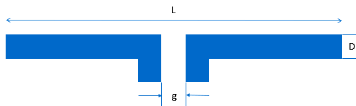
Figure 1: Plane view of Half-Wave Dipole Antenna.
