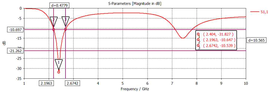
Figure 4: Bandwidth Curve for the designed Half-Wave Dipole Antenna.
