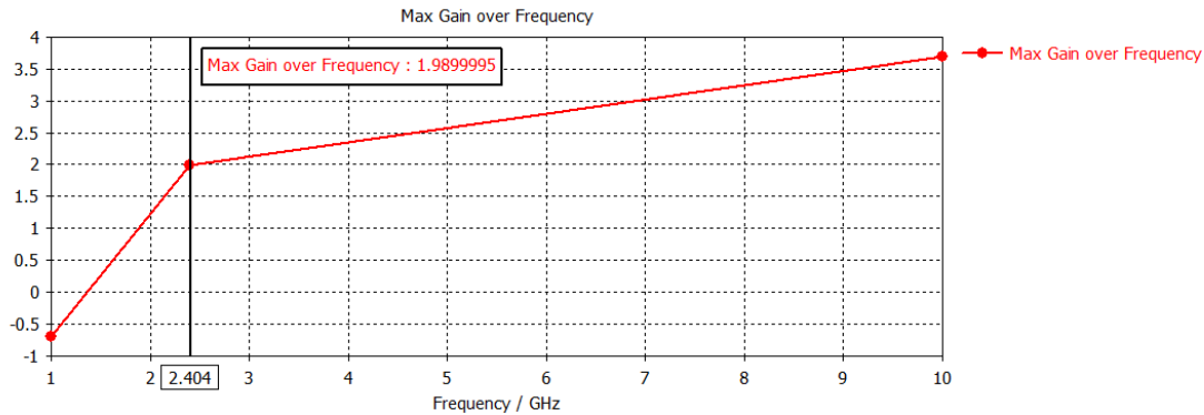
Figure 7: Max. Gain of the designed Half-Wave Dipole Antenna.
