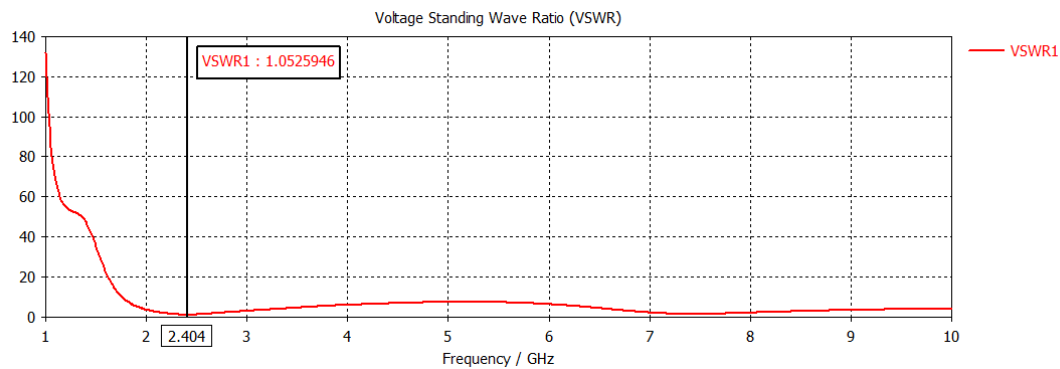
Figure 5: VSWR of the designed Half-Wave Dipole Antenna.
