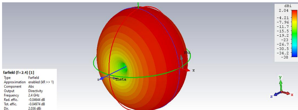
Figure 6: 3-D Radiation Pattern of Directivity for the designed Half-Wave Dipole Antenna.
