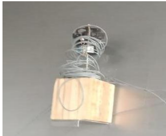
Fig.5. RTD PT 100 sensor fitted in wood core.
