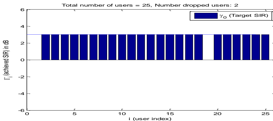
Figure 8: Achieved SIR for number of dropped users = 2.
