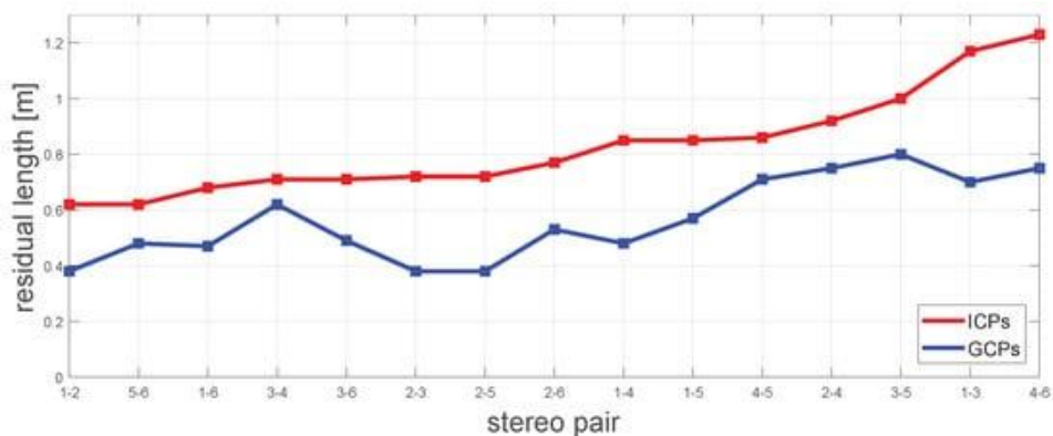
Figure 3: The 3D length discrepancies for the Ljubljana set sorted from lowest to highest ICP error. ICP values are given in red and corresponding GCP values in blue (Perko, et al, 2018).
