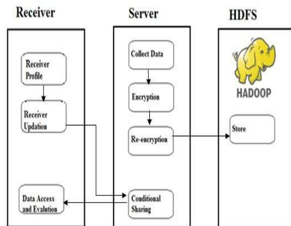
Figure 2: System Architecture.
