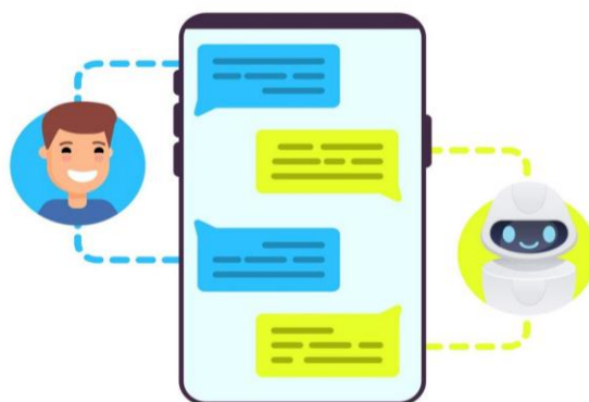
Fig 1: Chatbot.
