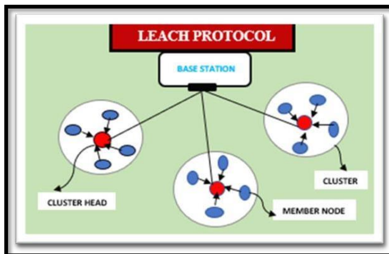
Figure 2: LEACH Protocol.
