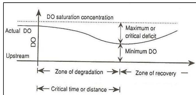
Figure 2.1: Typical changes in DO downstream of a wastewater input to a river.
