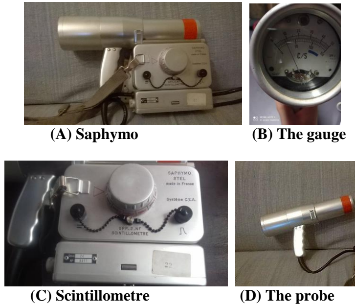
Fig. 2: The main components of the SAPHYMO radiation detector.
